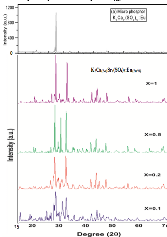
Fig. 1 XRD pattern of \text{K}_2\text{Ca}_{2-x}\text{Sr}_x(\text{SO}_4)_3 with different contents (x) of Sr.
