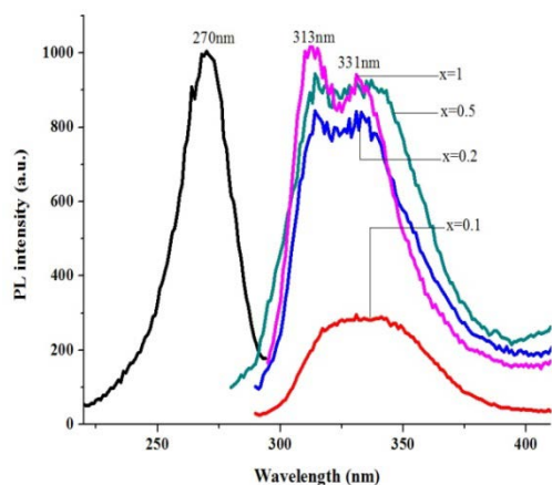
Fig. 7 PL spectra of \text{K}_2\text{Ca}_{(2-x)}\text{Sr}_x(\text{SO}_4)_3:\text{Ce}_{(5\text{m}\%)} monitored at 270nm excitation. ( \lambda_{\text{emi}}=313\text{nm} )
