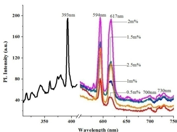
Fig.3. PL spectra of KCSS: \text{xEu}^{3+} phosphor monitored at 393nm excitation. Fig. 4 PL spectra of \text{K}_2\text{Ca}_{(2-x)}\text{Sr}_x(\text{SO}_4)_3:\text{Eu}_{(2\text{m}\%)} phosphor monitored at 393 nm excitation.
