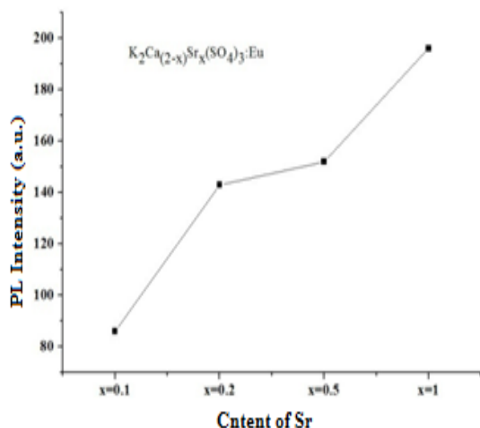
Fig. 5 Change in PL intensity with variation of \text{Sr}^{2+} content in \text{K}_2\text{Ca}_{(2-x)}\text{Sr}_x(\text{SO}_4)_3:\text{Eu}_{(2\text{m}\%)} .
