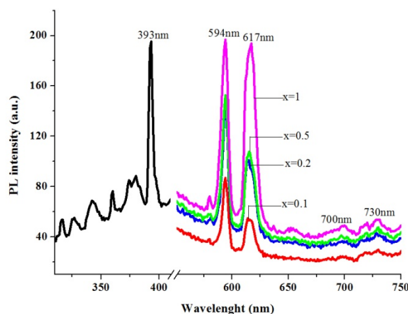
Fig.3. PL spectra of KCSS: \text{xEu}^{3+} phosphor monitored at 393nm excitation. Fig. 4 PL spectra of \text{K}_2\text{Ca}_{(2-x)}\text{Sr}_x(\text{SO}_4)_3:\text{Eu}_{(2\text{m}\%)} phosphor monitored at 393 nm excitation.
